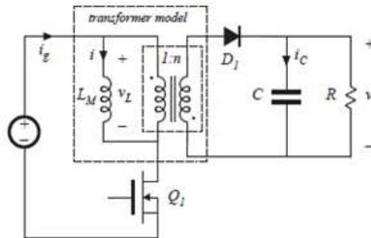
(a) A comparable flyback converter transformer circuit is modeled.
