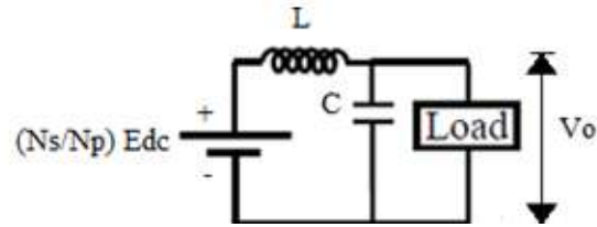
(b) shows the Mode-1 comparable circuit.
