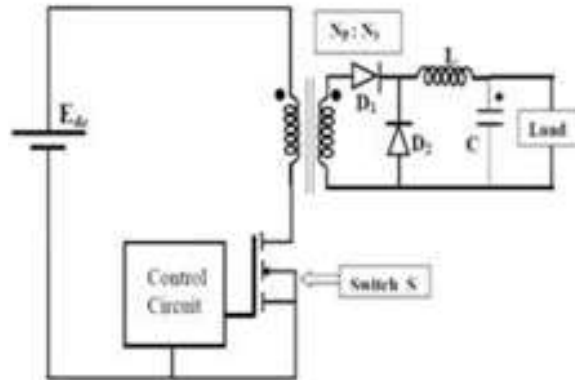
Figure4:The forward converter's essential construction
