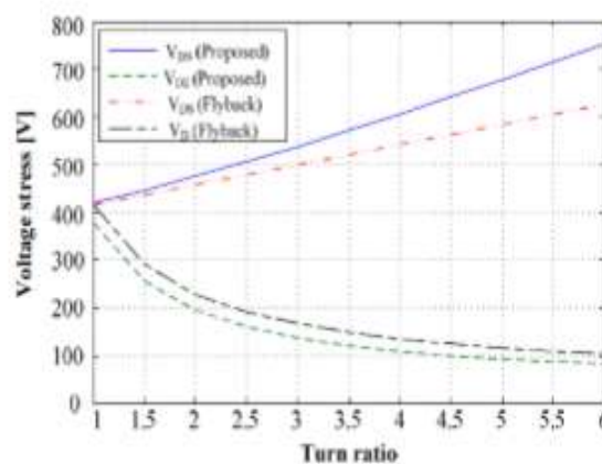
Figure 8: The voltage stresses in forward-flyback and standard flyback converters are compared.
