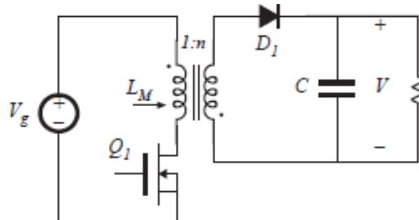
(d) having a positive output and a 1:n input-to-output ratio.
