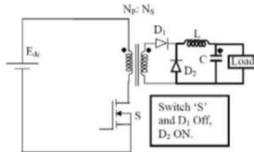
(a) Mode-2 is the current lesson.
