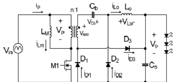
Figure7:The circuit diagram depicts the proposed forward flyback converter.
