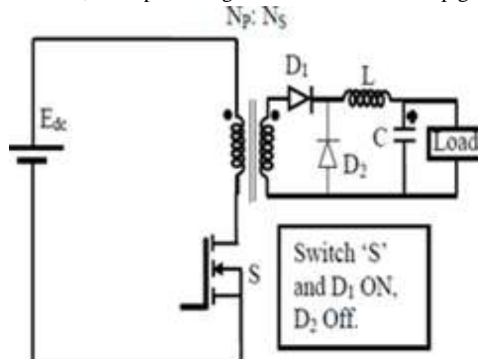
(a) Mode-1's current state.
