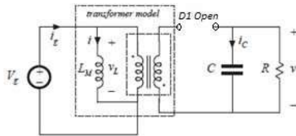
(b) If diode D1 is turned off.
