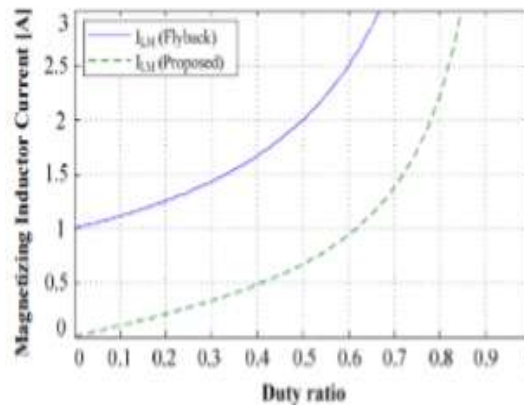
Figure 9: The magnetizing offset currents of a typical flyback converter are determined by the duty ratio.
