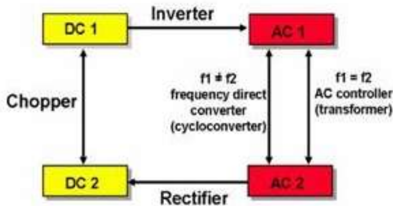
Figure1: The categorization of converters
