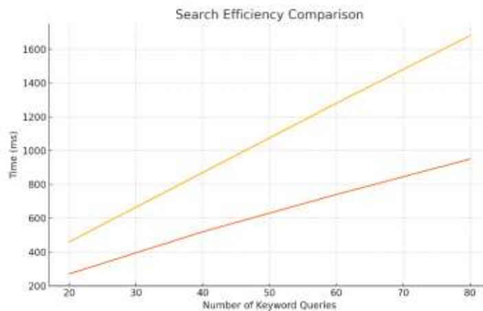
Figure 2. Keyword search query time comparison showing superior performance of CPAB-KSDS.
