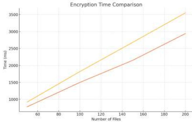
Figure 1. Encryption time comparison between existing system and CPAB-KSDS framework.
