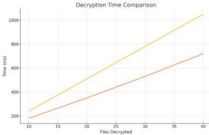
Graph 3: Decryption Time Analysis
